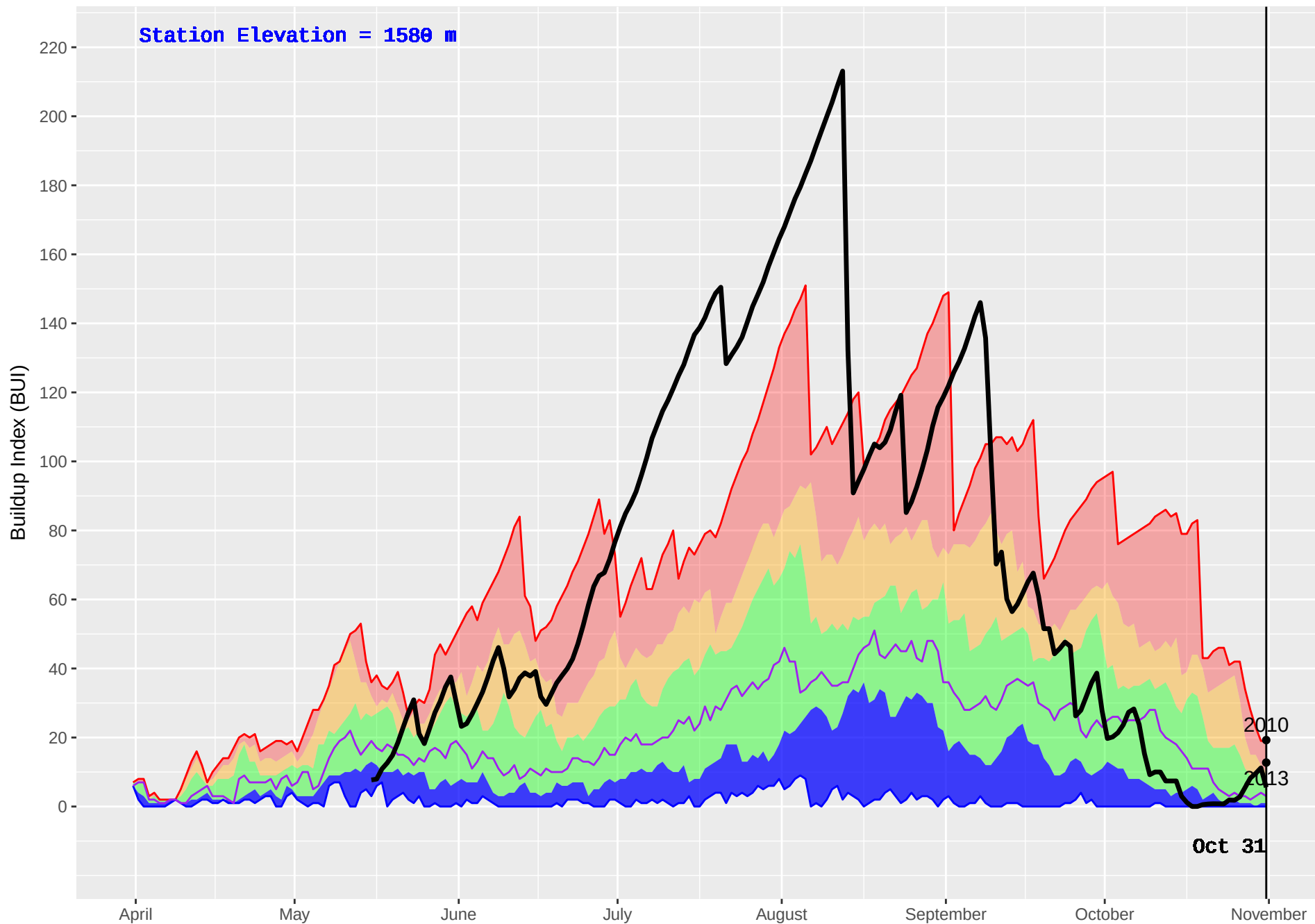
WINDY MOUNTAIN (244) : Historical (1989–2016) and Current (2017) Noon Buildup Index (BUI)
