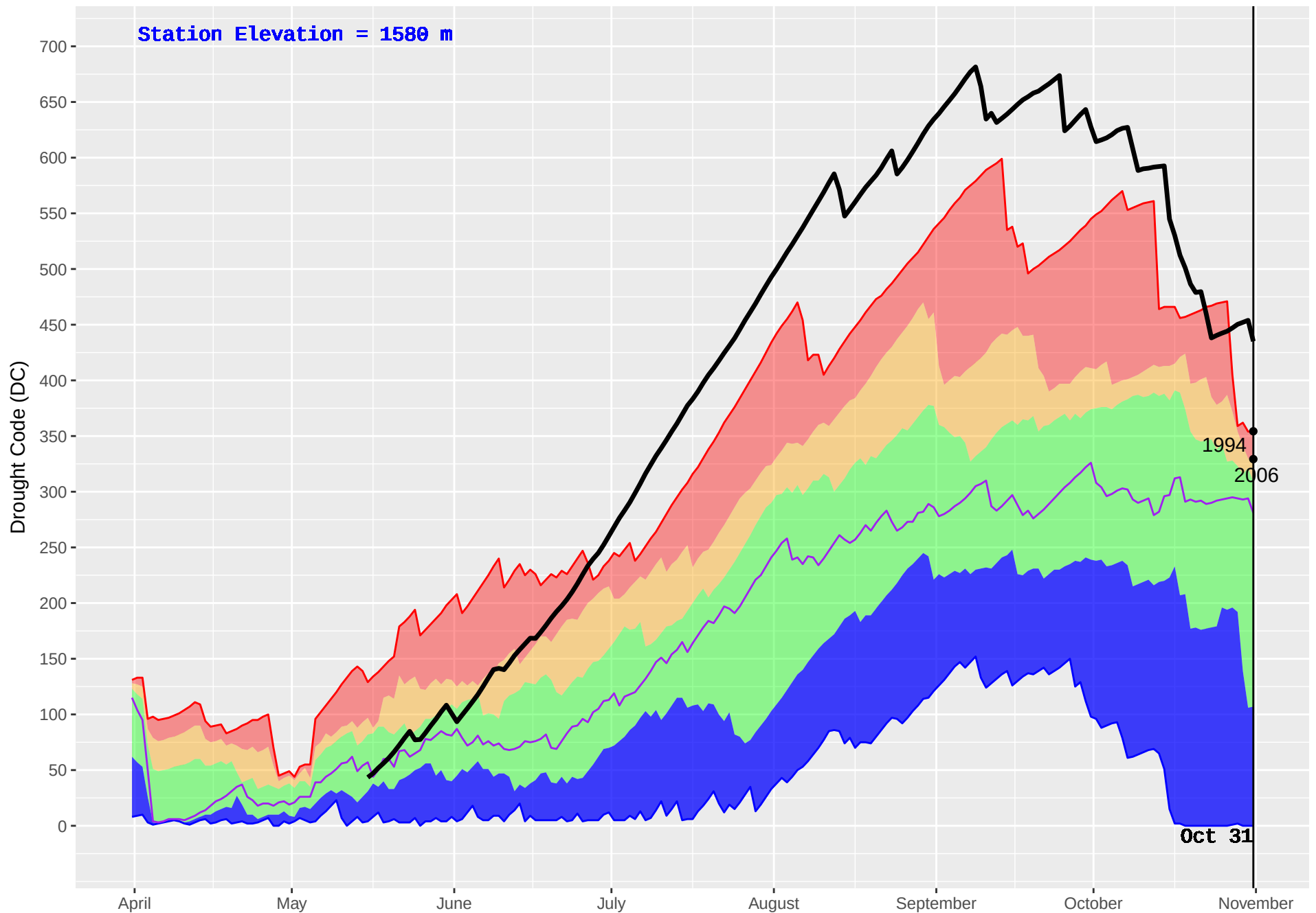
WINDY MOUNTAIN (244) : Historical (1989–2016) and Current (2017) Noon Drought Code (DC)
